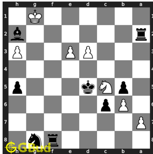
Figure 4: Bh2+
