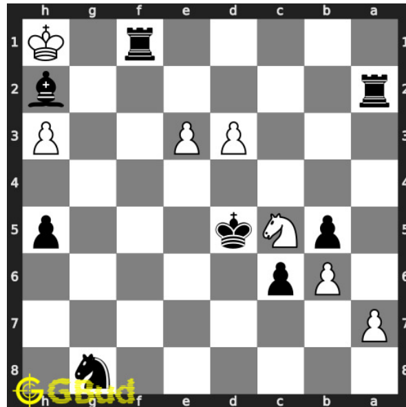
Figure 6: Rf1#
